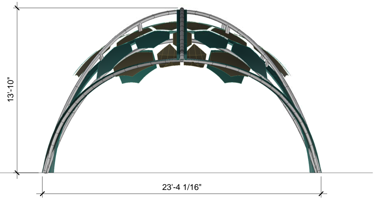
3 TURTLE POD SIDE SCALE: 1:60
