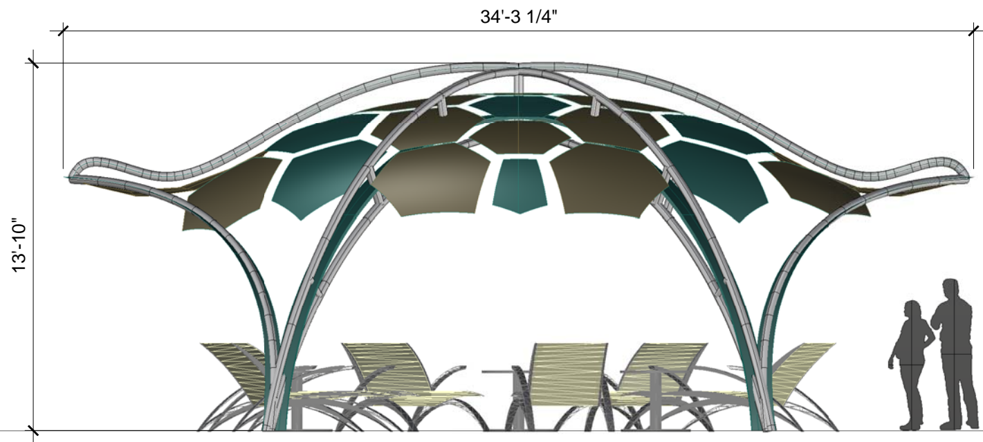
1 TURTLE POD FRONT SCALE: 1:60
